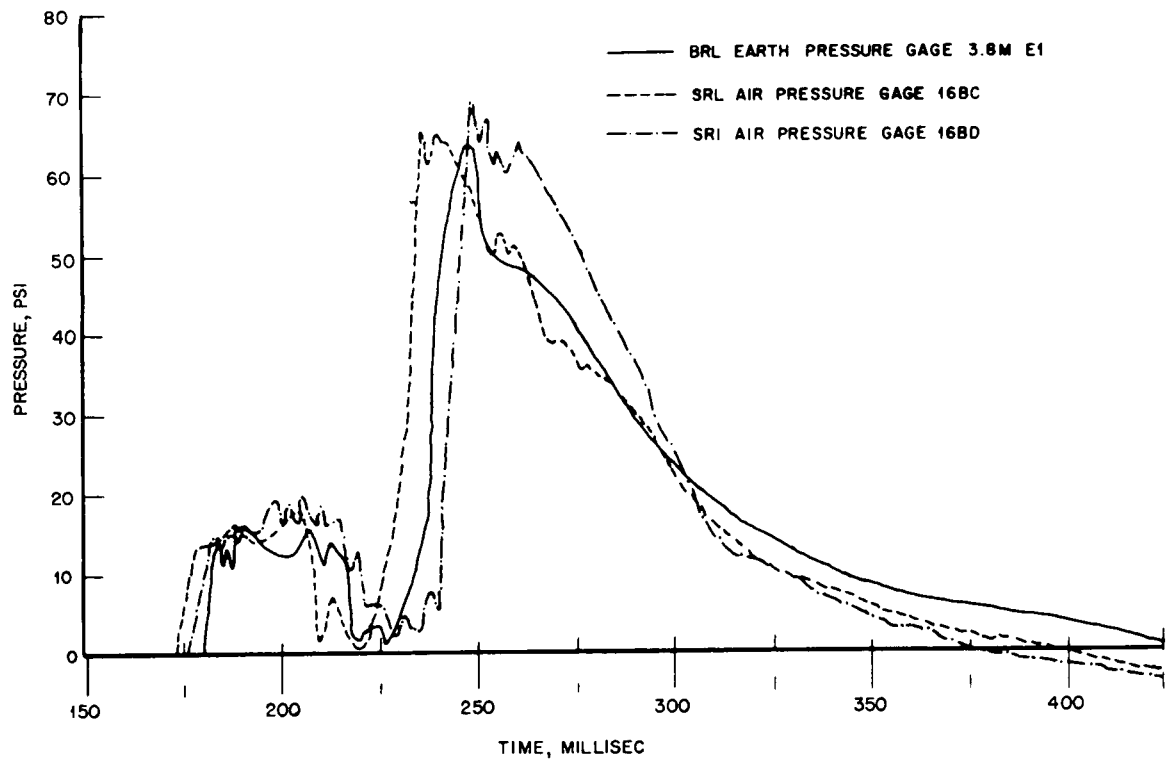
Fig. 9—Pressure on ground surface, shot 10.
